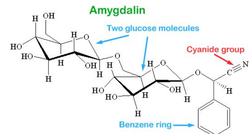
Figure 1. Structural model of amygdalin.
